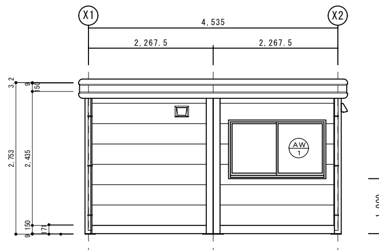
Y2側立面図 S = 1 / 5 0
